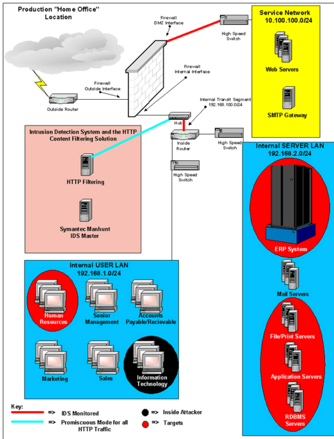
Figure 5 Theoretical Network
