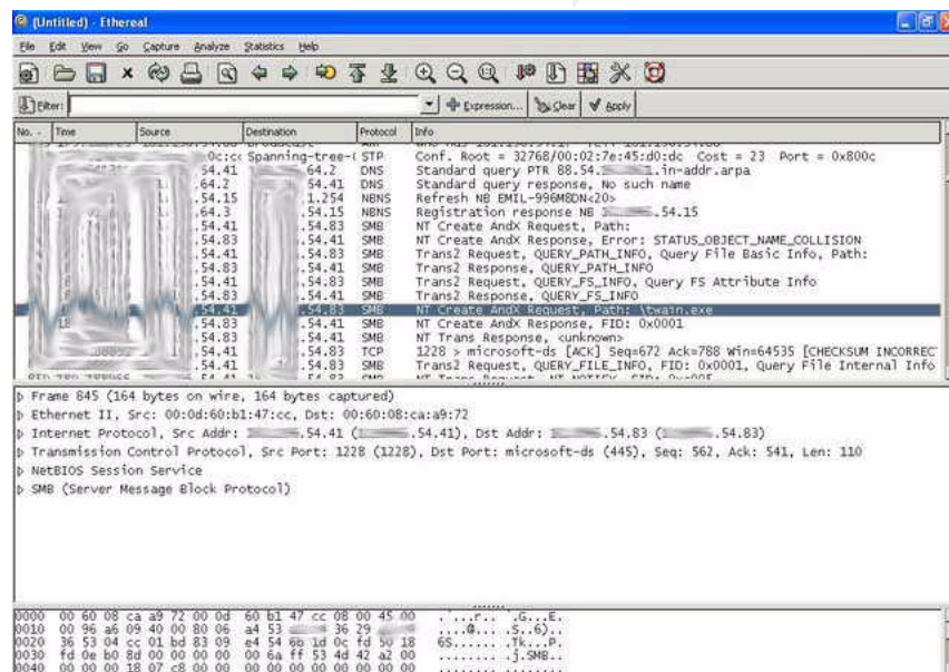
Figure 26. twain.exe found in the ethereal capture
