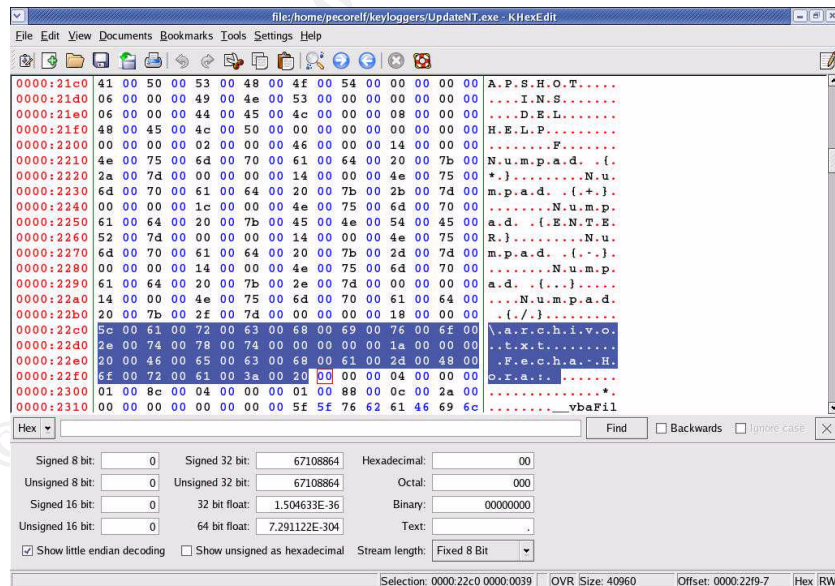
Figure 15. Words found with khaxedit
