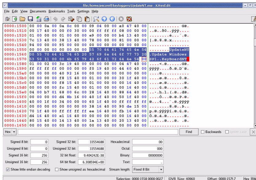
Figure 14. Opening UpdateNT.exe with khxedit
