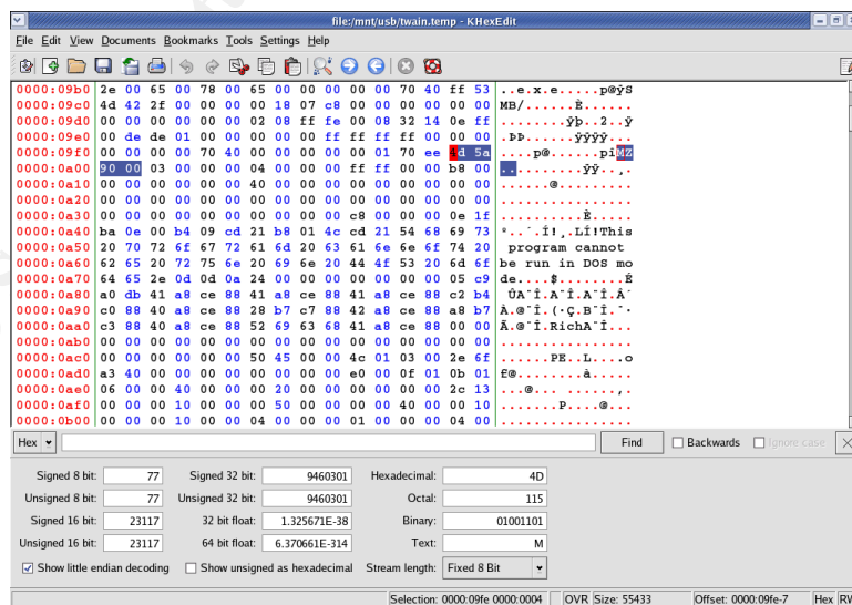
Figure 29. Header of executable file found in the transfer
