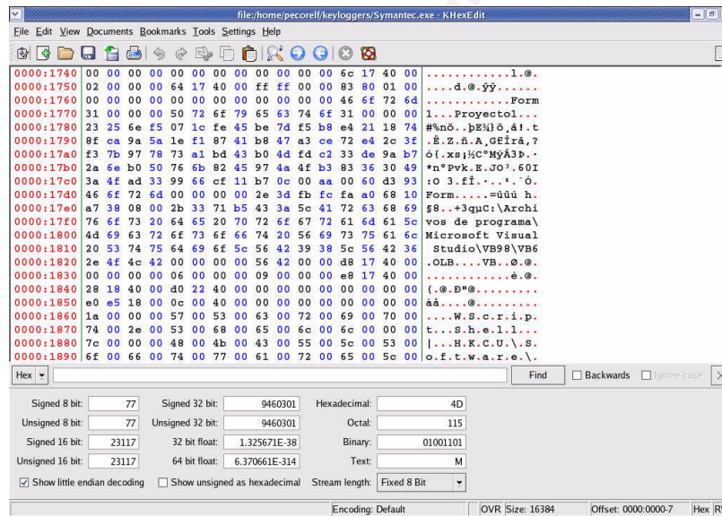
Figure 11. A view of Symantec.exe using khexedit (Continuation)
