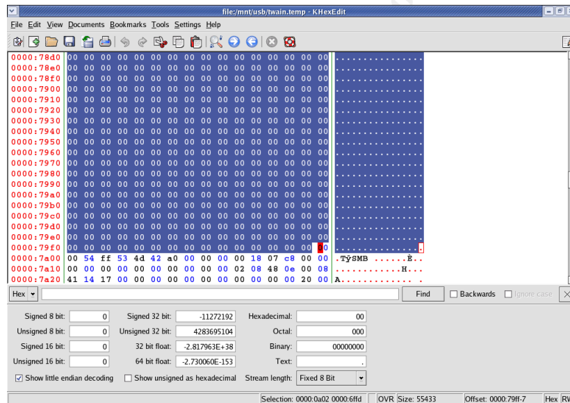
Figure 31. Extracting twain.exe from the transfer
