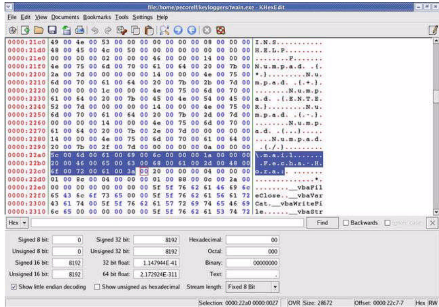
Figure 22. Presence of mail call and the tag Fecha - Hora
