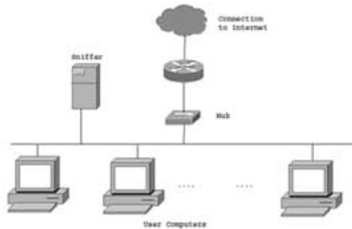
Figure 4. Net configuration of the commercial offices
