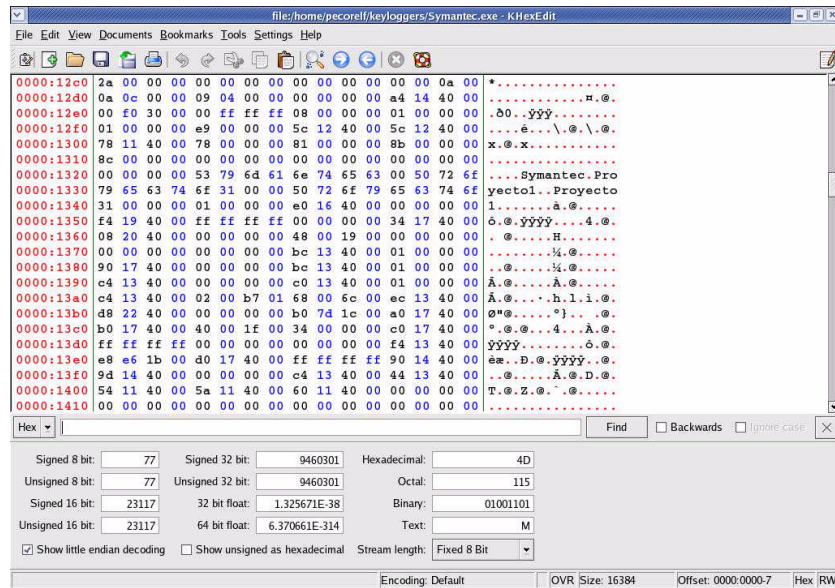
Figure 10. A view of Symantec.exe using khexedit
