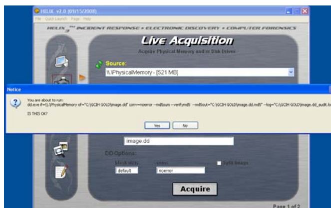
Figure 30 – Helix Live Acquisition Prompt.
