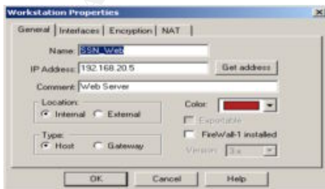
Figure 2 – Checkpoint Object
