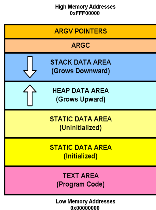
Figure 1 The Structure of Program Memory
