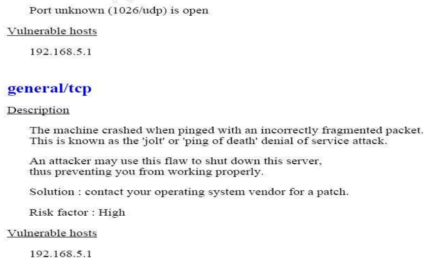
Figure 18 Sample report - "ping of death" vulnerability.
