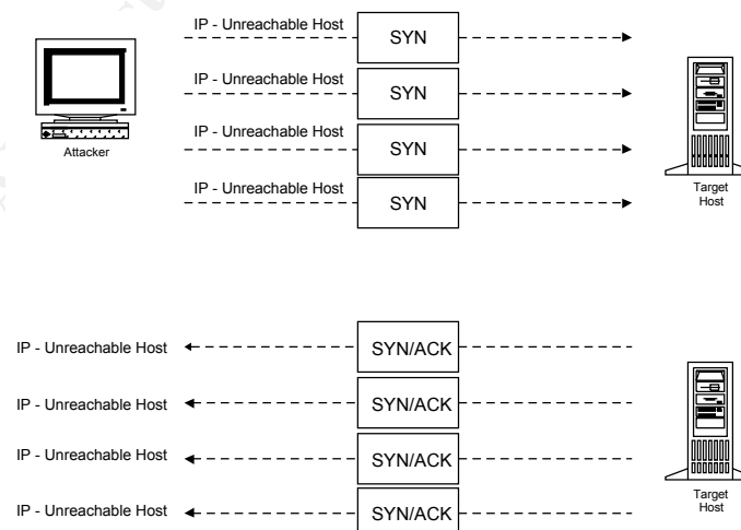
Figure 2. SYN Flood
