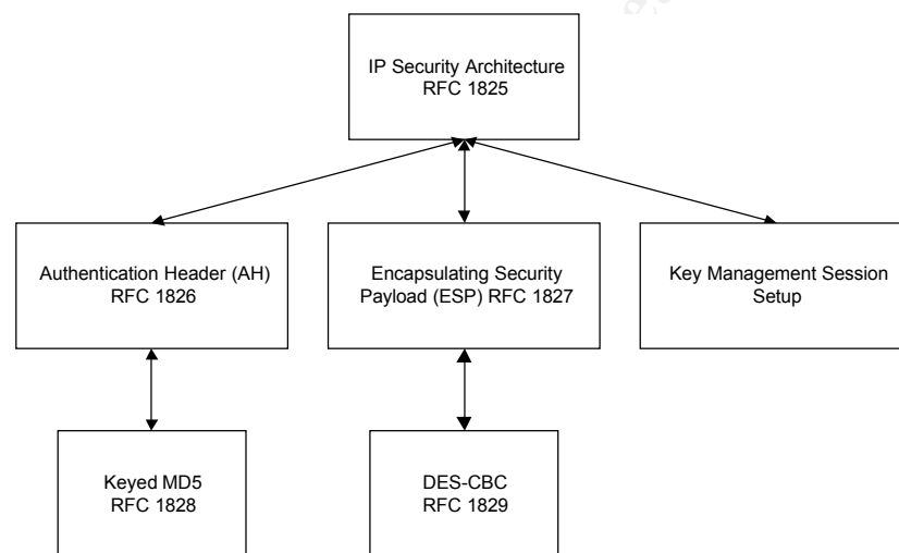
Figure 5. IPsec Structure
