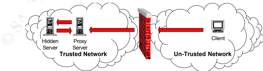
Figure 4. Proxy Server
