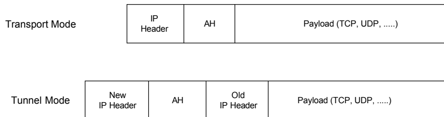
Figure 6. AH Format
