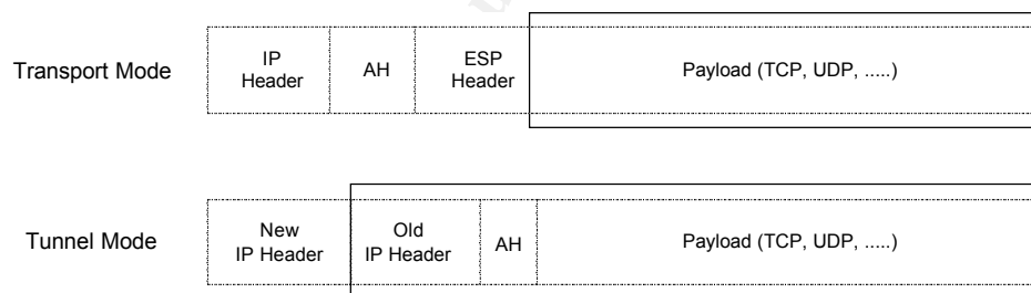
Figure 7. ESP Encapsulation
