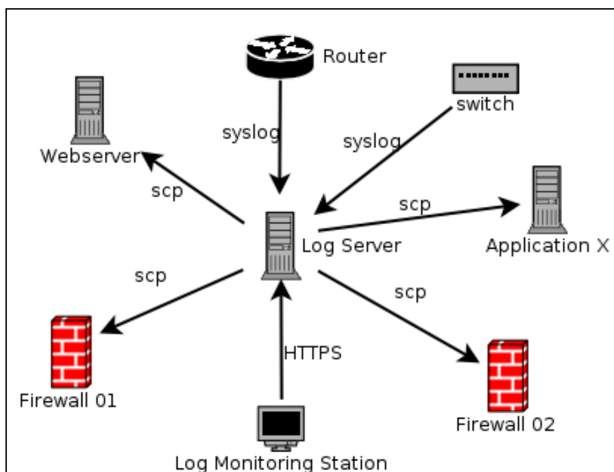
Illustration 2: Overall Architectural Log Collection Diagram
