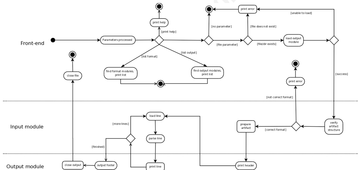
Figure 2: UML chart showing the process of log2timeline, main CLI front-end
