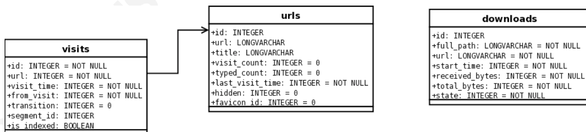
Figure 6: Shows the relationship and structure of three tables in the Chrome History database
