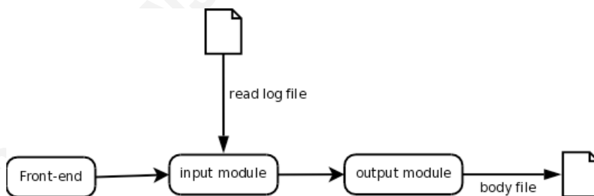
Figure 1: A simple flow chart of the structure of log2timeline
