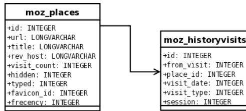
Figure 7: Relationship schema for the two of the tables in places.sqlite SQLite database
