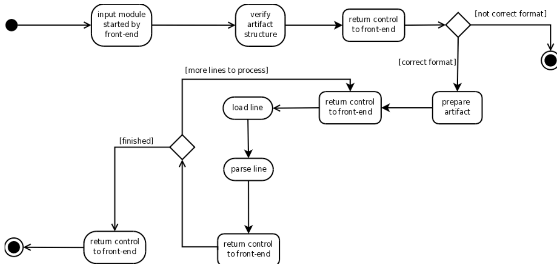
Figure 4: Shows the flow of operation for an input module
