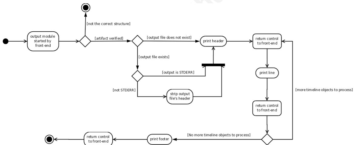
Figure 5: The flow of operation for the output module
