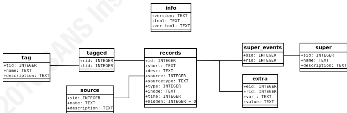
Figure 11: Shows the database schema for the SQLite database output
