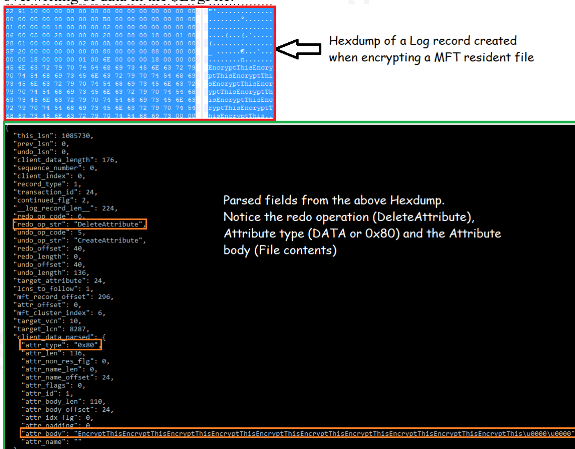
Figure 6-3 – The NTFS $LogFile showing contents of a MFT resident file.
