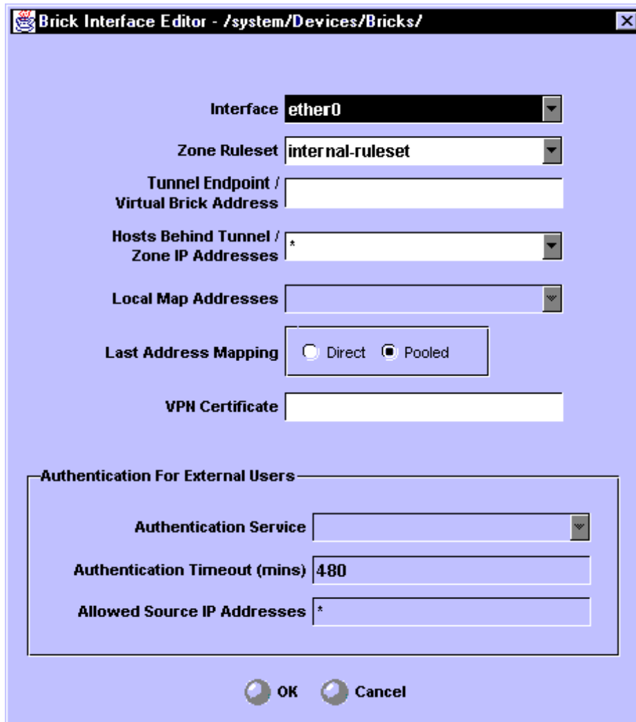
Figure 10 Interface Editor
