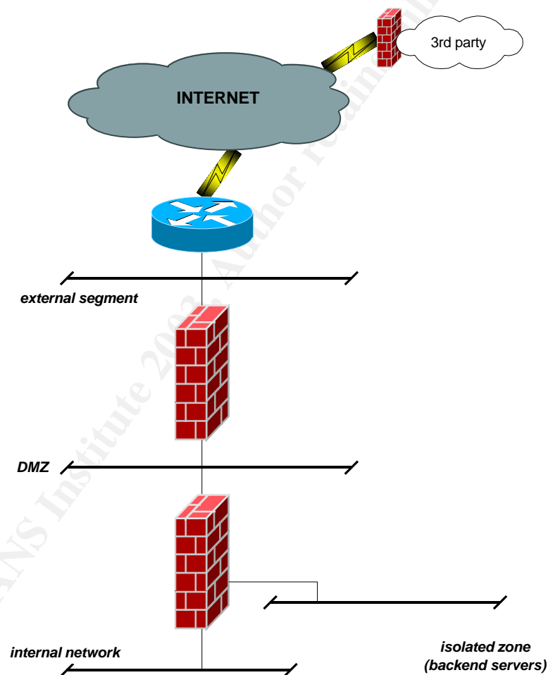
Figure 3. Alternative Architecture
