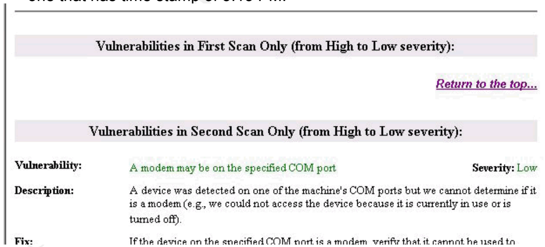
Figure 16 Differential Report Sample
