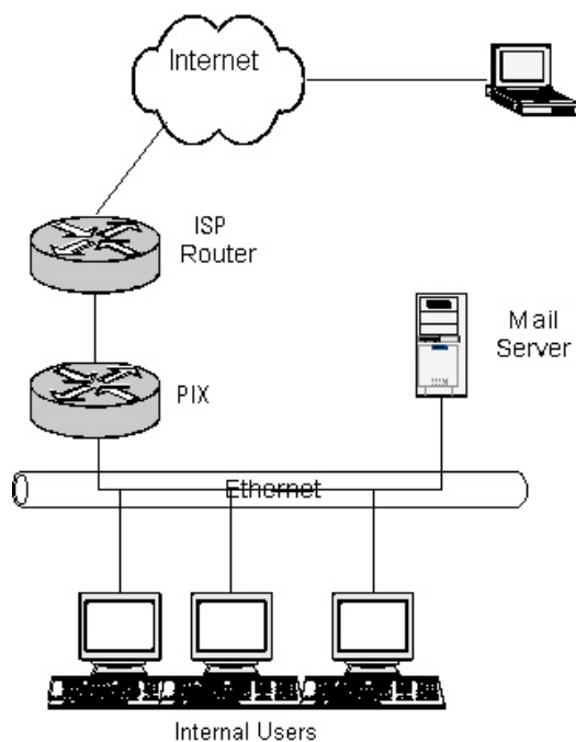
Figure 3- Typical Small office configuration
