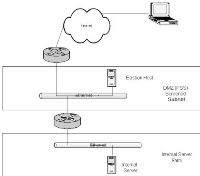
Figure 4- Typical bastion host configuration
