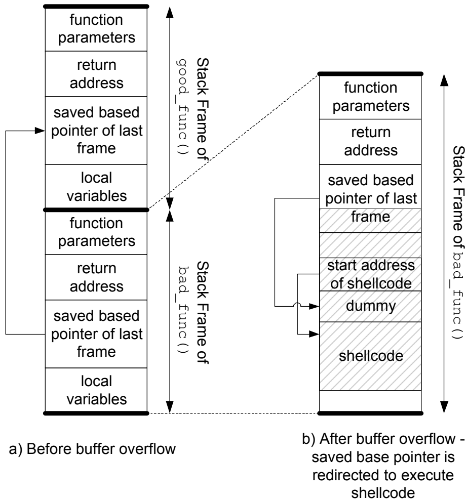
Figure 9: Exploiting off-by-one errors
