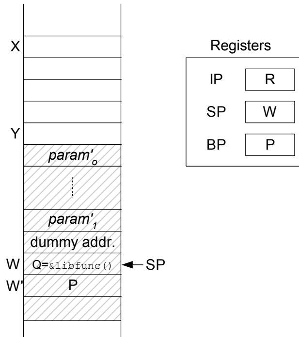
Figure 10: Return-into-libc exploit
