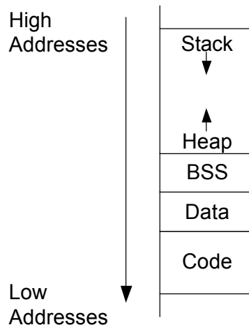
Figure 1: Memory layout of a binary (adapted from [24])
