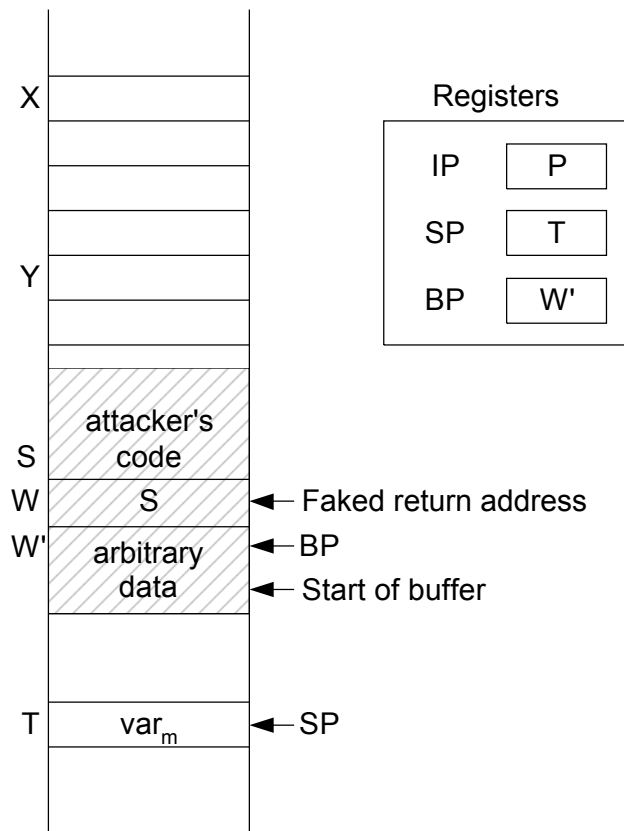
Figure 6: Stack after buffer overflow
