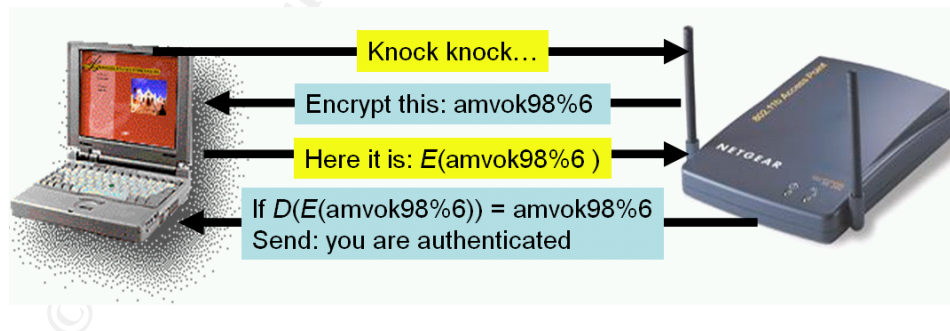
Figure 2. Shared-Key Authentication
