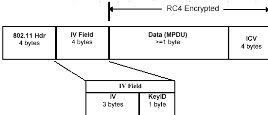
Figure 4: WEP-encoded MPDU [16].
