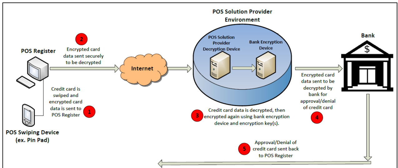
Figure 3 – P2P Encryption Data Flow
