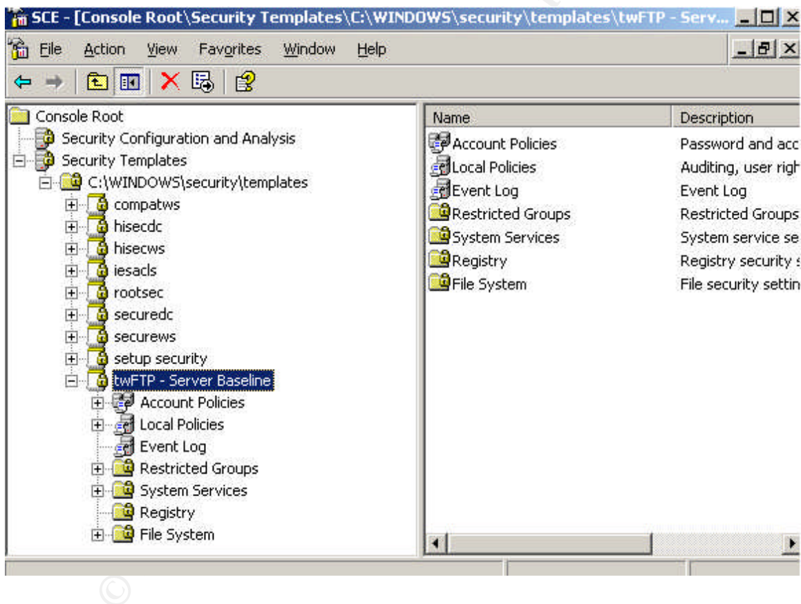
Figure 4 – Security Templates
