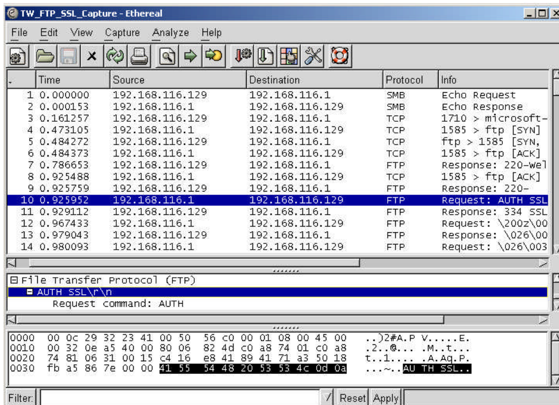
Figure 14 – Ethereal 26 trace showing Explicit FTPS connection sequence
