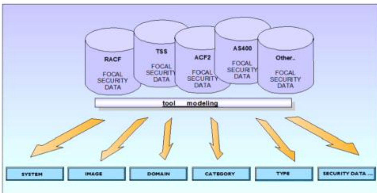
Figure 5: Data modeling
