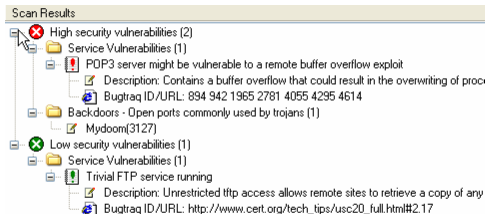
Figure 26 LanGuard NSS reported false positives
