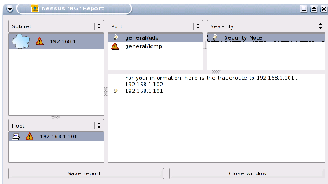
Figure 27 No vulnerability noted on UDP
